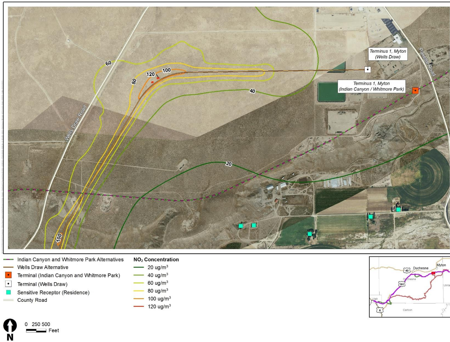
Figure 3.7-5. Maximum 1-Hour NO 2 Concentrations South of Myton (Wells Draw Alternative)
