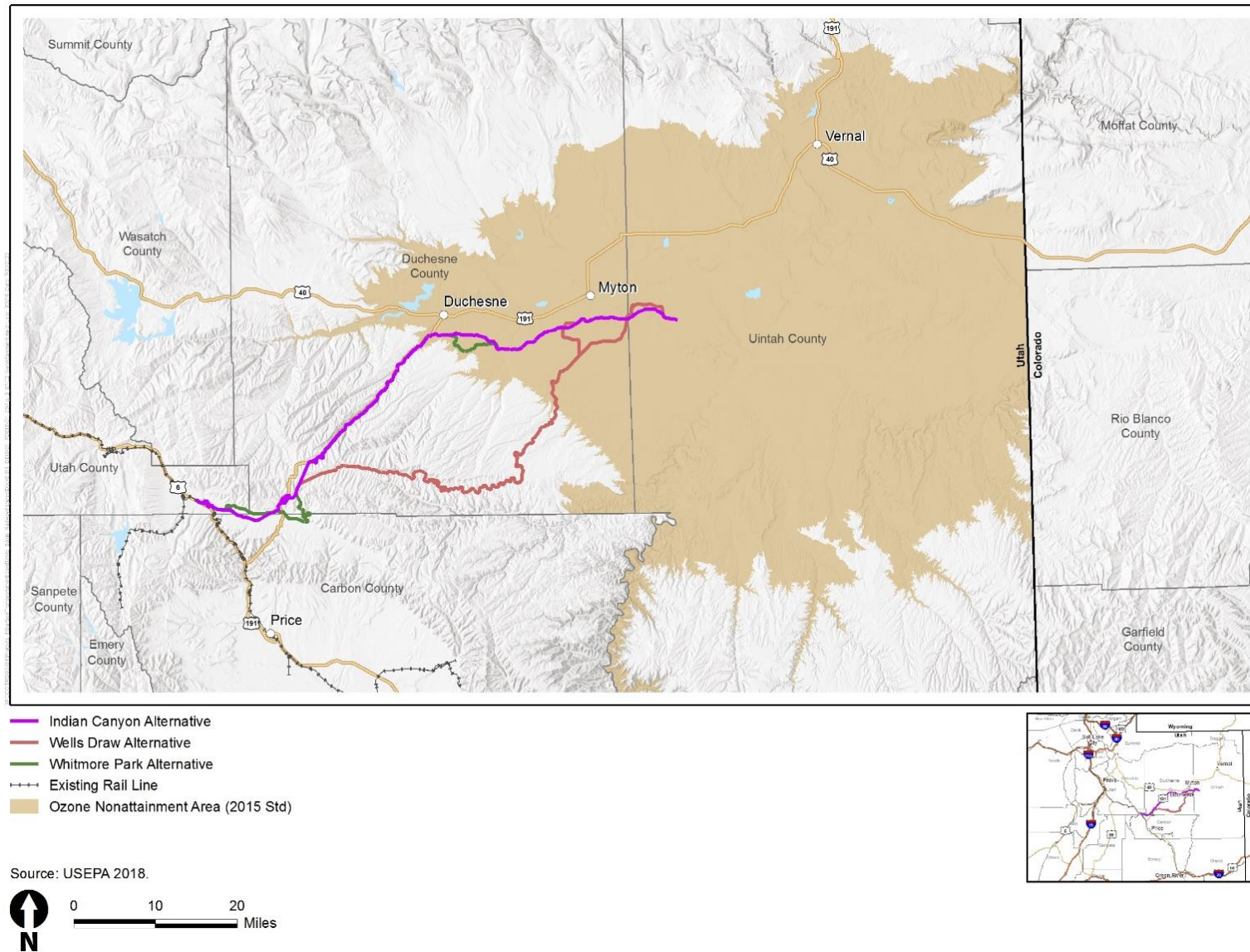
Figure 3.7-2. Ozone Nonattainment Area
